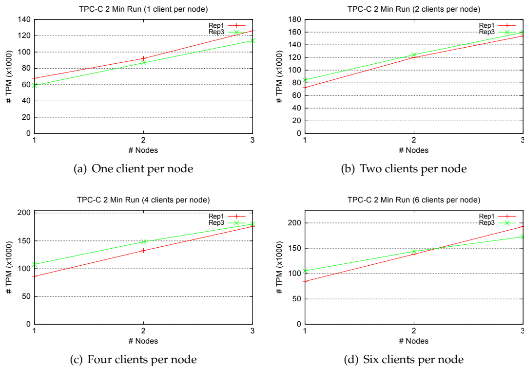
Figure 5.10: Multi-core results
