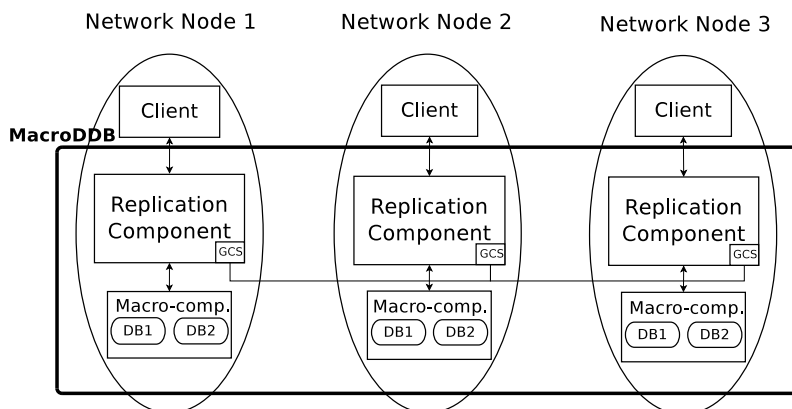
Figure 4.1: MacroDDB Deployment Architecture
