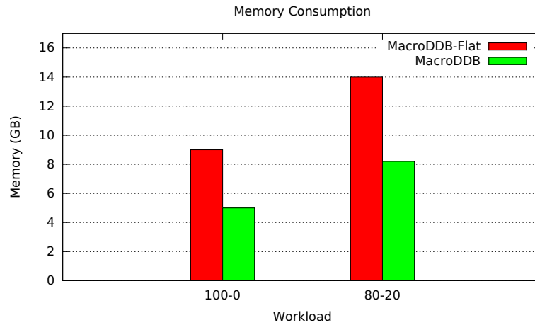
Figure 5.4: Memory usage
