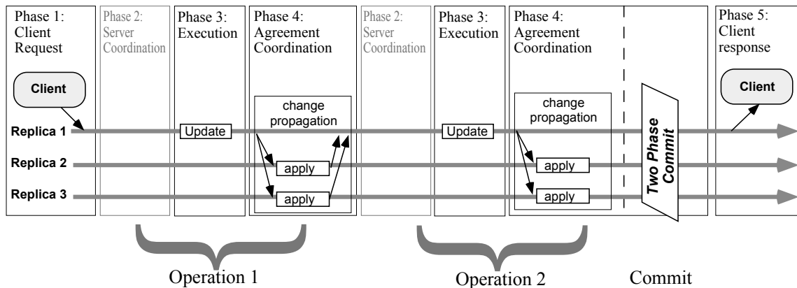
Figure 2.3: Eager primary copy (taken from [Wie+00a])
