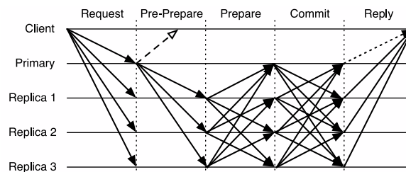
Figure 2.12: PBFT-CS early reply (taken from [Wes+09])
