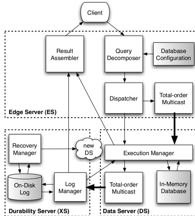
Figure 2.9: Sprint architecture (taken from [Cam+07])
