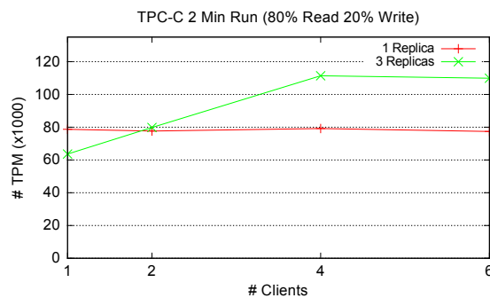
Figure 5.9: MacroDB performance sample
