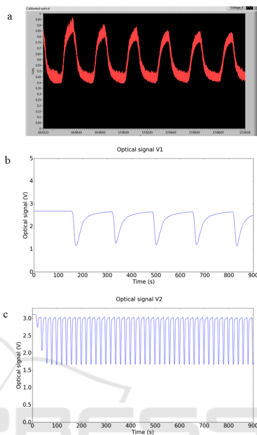
Figure 7: Evolution of optical signals from (a) E-nose V0 to (b) E-nose V1 and (c) E-nose V2. The gas sample used was atmospheric air saturated in acetone for all the plots.
